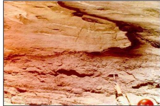
Figure 11. Photo of Shirley Basin Roll Front
